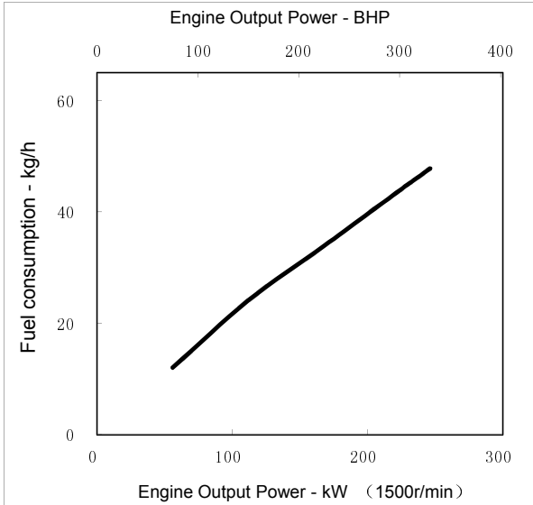
Engine Performance Data @ 1500rpm
